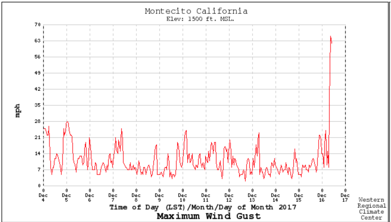
Figure 4 Maximum wind gust
